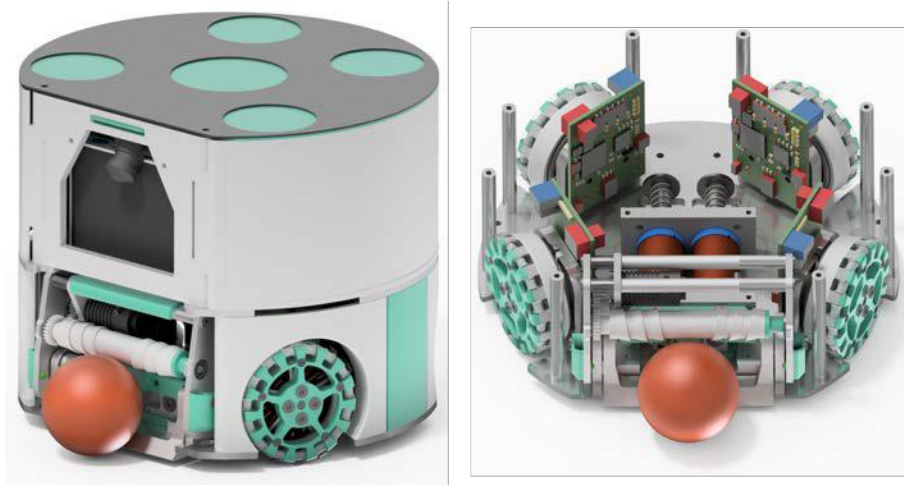
Fig. 1: GreenTea robot design from 2022.
