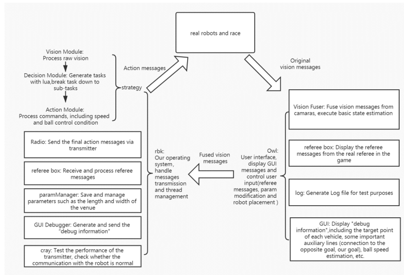
Fig. 11. Workflow of our technical framework in real game mode
