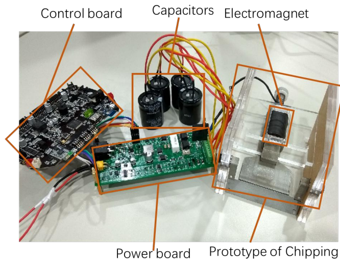
Fig. 5. Test system
