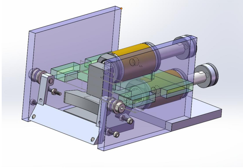
Fig. 3. Prototype of kicking and chipping part
