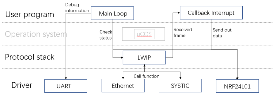
Fig. 8. Overall structure of transmitter
