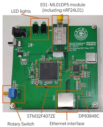
Fig. 9. PCB board for network transmitter
