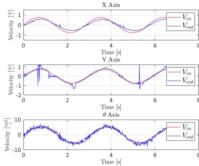
Fig. 6. Harmonic Analysis.
