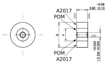
Fig. 5. A hub of a small wheel (after replacing)
