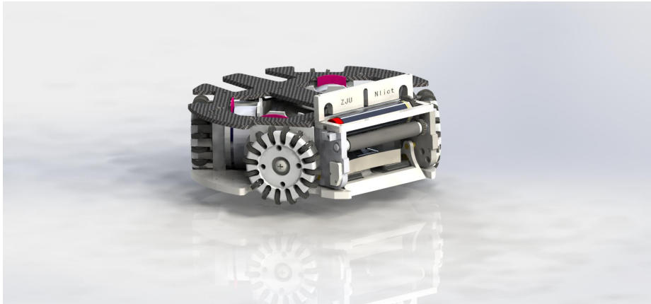
Fig. 1. Overall Mechanical Structure
