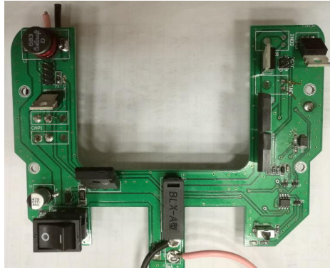
Fig. 5. A Demo for New Power Board
