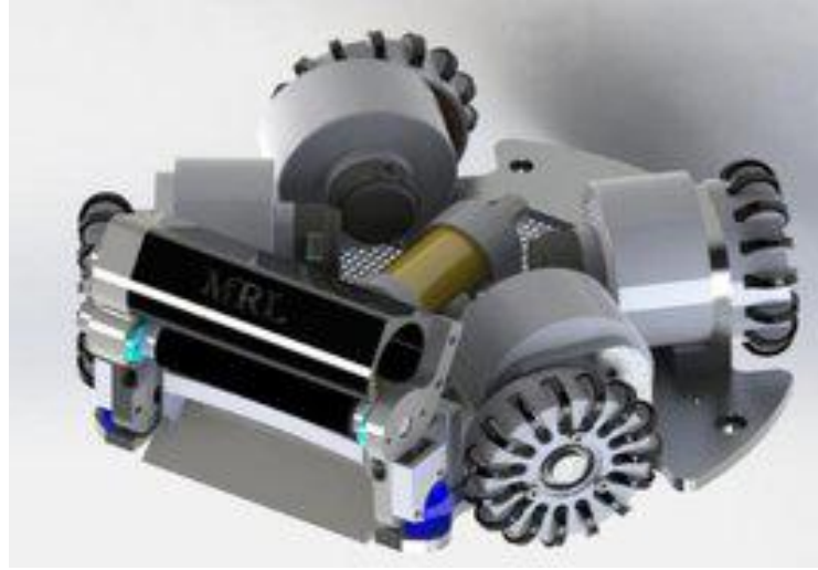
Fig. 17. Robot 2015 mechanical structure
