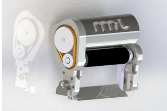
Fig. 21. New dribbling system of the MRL robot
