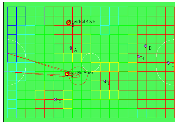
Fig. 11. Applying the rule (C)
