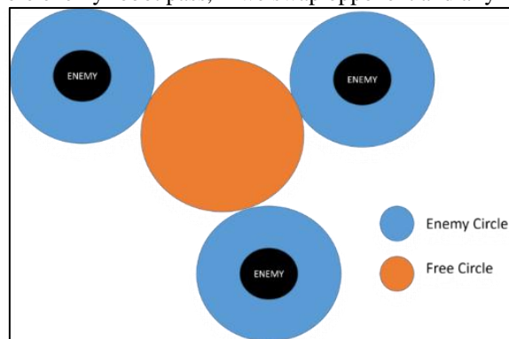
Fig. 8. Enemy Circle and Free Circle
