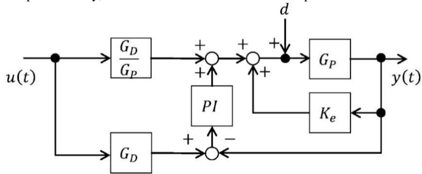
Fig. 6. Block diagram of control circuit
