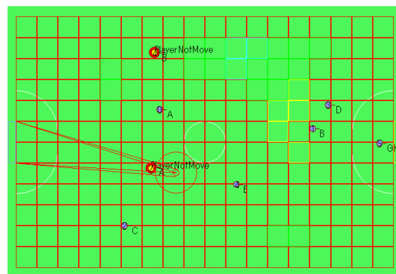
Fig. 12. Applying the rule (D), (E) and (F)
