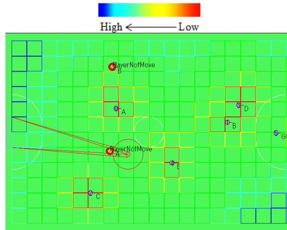
Fig. 10. Applying the rule (A) and (B)
