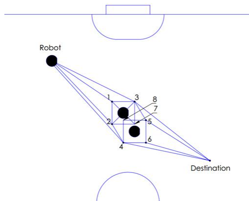
Figure 7: Pathplanning graph
