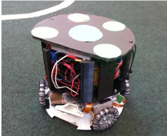
Fig. 3. First generation RoboBulls SSL robot.
