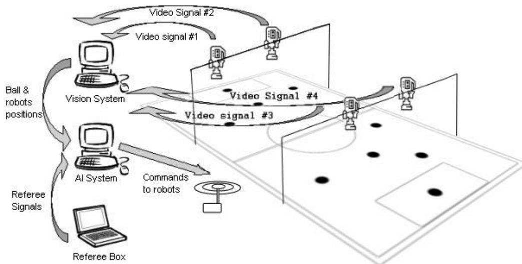
Fig. 1. Typical architecture of a SSL team.
