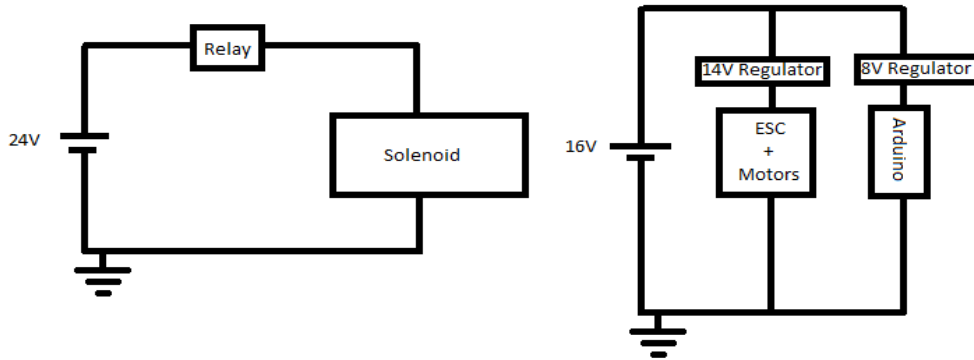
Fig. 4. Power supply to robot components
