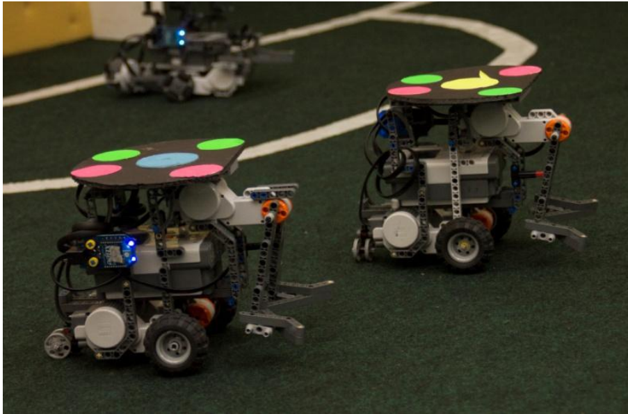
Fig. 5. Lego NXT Robots used for initial development
