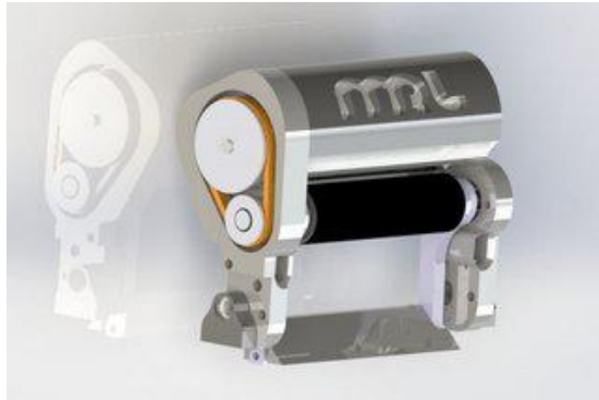
Fig. 19. New dribbling system of the MRL robot
