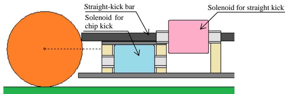
(a) The height of straight-kick bar (previous)
