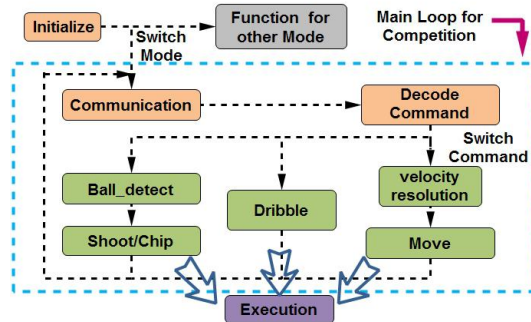
Fig. 2. Embedded software flowchart
