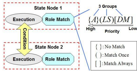
Fig. 7. FSM-based Role Match Framework. A role match item’s syntax is described on the right: the letter in the string is short for the role’s name in the state node(A-Assister, L-Leader, S-Special, D-Defender, M-Middle). We offer three modes for matching, No Match means to keep the role as same as last state, Match Once means match the role once stepping into this state, and Match Always means do role match every cycle. If a robot is missing, then ignoring the last role in the item and No Match group always has a higher priority.
