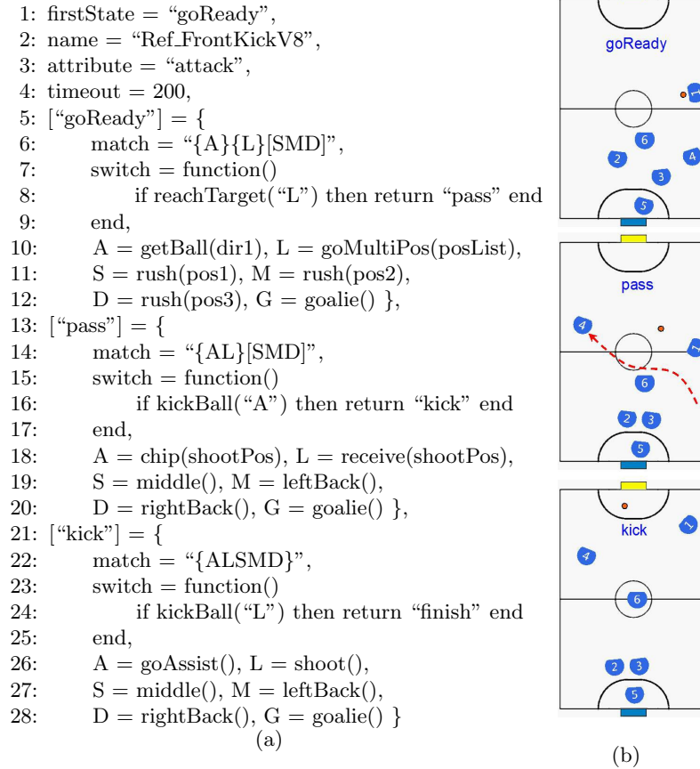
Fig. 5. An example of indirect free kick in frontcourt: (a) Lua script; (b) positions of robots in every state. In the script (a), the basic settings are from line 1 to line 4. Then we define the specific states in this play. For example, the state goReady comprises a role match item (line 6), switch condition (line 7-9) and execution (line 10-12).
