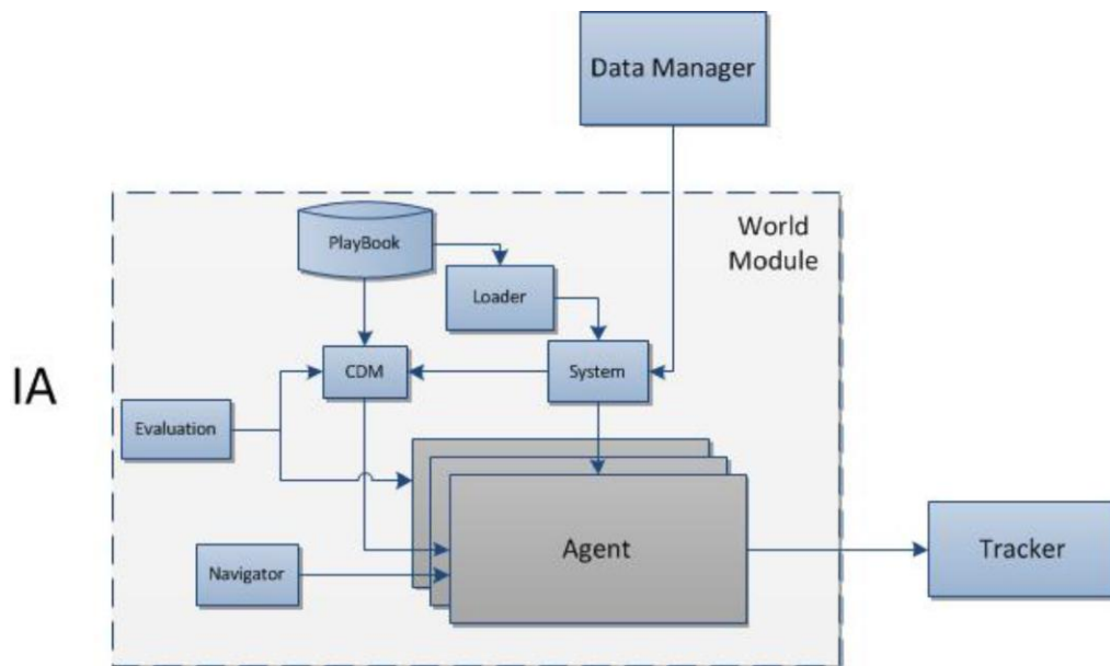
Fig. 4. Software Design.
