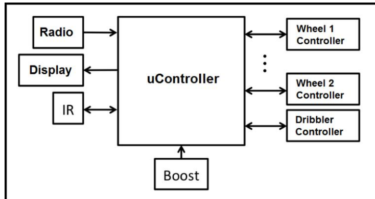
Fig. 2. Overview of Embedded Architecture.
