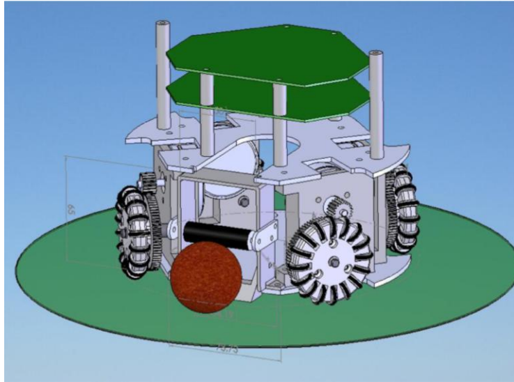
Fig. 1. Mechanical Structure.
