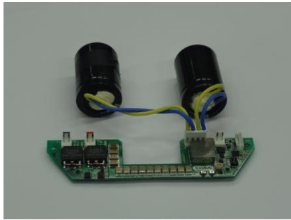
Fig. 4. Boost converter
