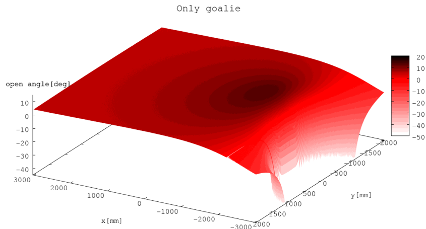
Fig. 16. Open angles computed by Algorithm 1
