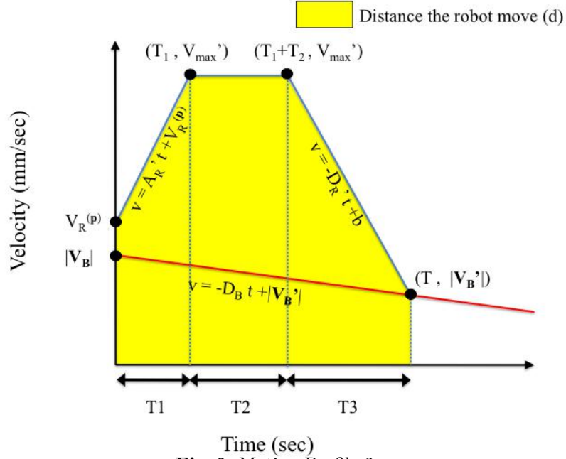
Fig. 9. Motion Profile 2
