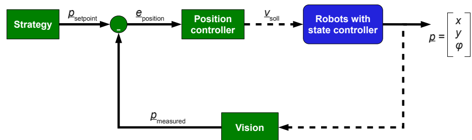
Fig. 3. Complete controller structure.
