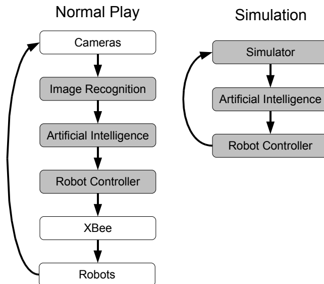
Fig. 3: Software Components
