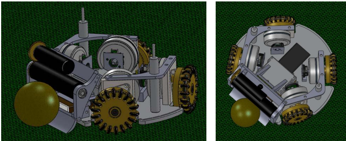
Fig.2. Robot's mechanical plan design.
