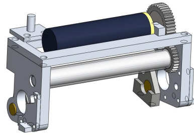
Fig. 6. Dribbling Device
