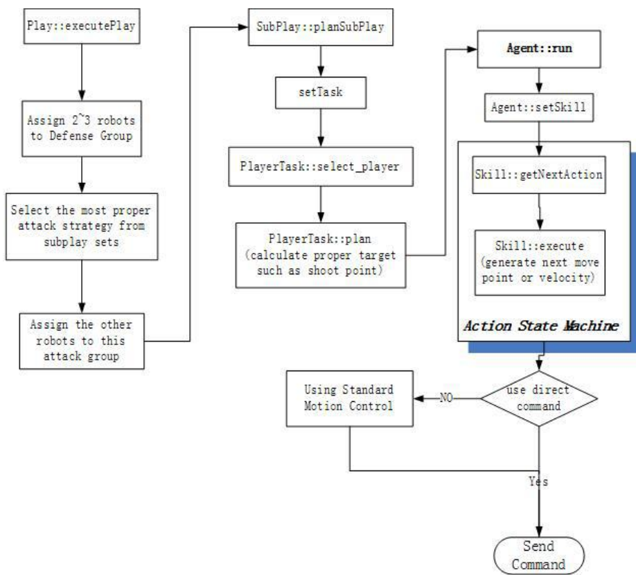
Fig. 17. Decision Routine
