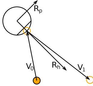
Fig. 11. The model for one-touch pass-and-shoot. The final velocity of the ball v_1 contains a component of the initial velocity v_0 , and thus is not parallel to the robot heading R_h .
