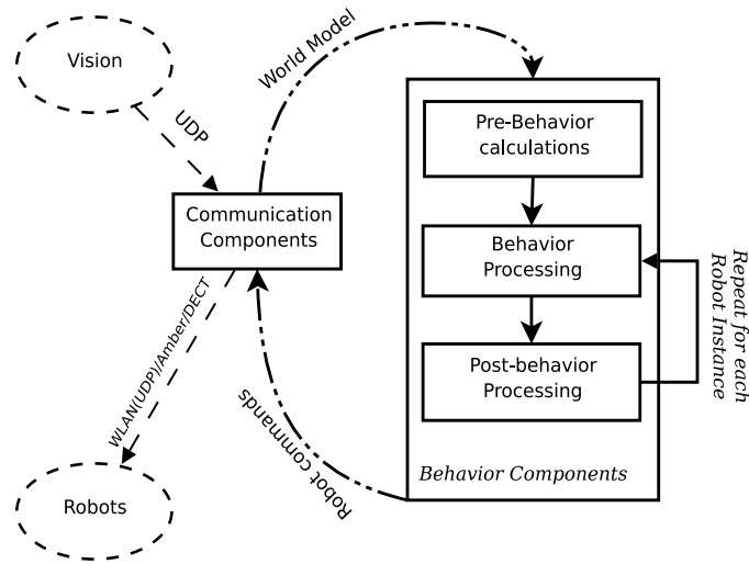
Fig. 3. Main loop structure of the agent software
