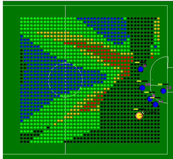
Fig. 4. Visualization of the yellow team’s position rating grid, showing good positions in red.
