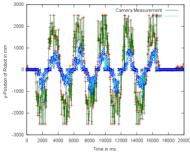
Fig. 2. Comparison of direct camera measurement and filtered value while performing sinus-shaped movement in y-direction
