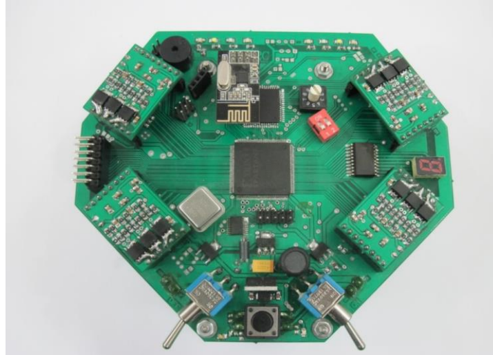
Figure 3. Main Board
