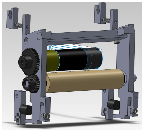
Fig. 1: 2012 Dribbler Design
