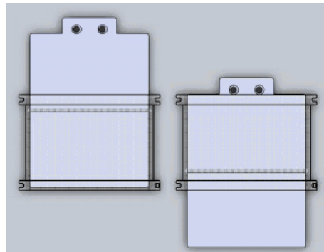
Fig. 2: Kicker solenoid at the beginning of the stroke (left) and end of the stroke (right)
