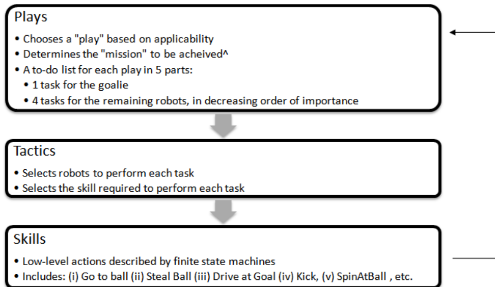
Fig. 4: 2012 STP Model
