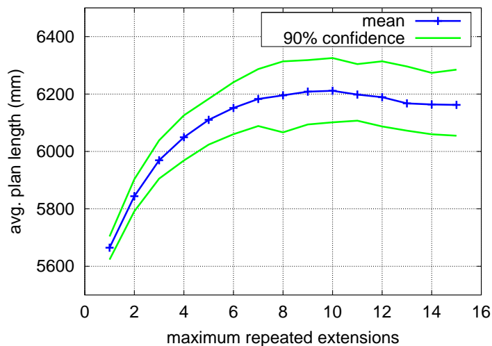
Fig. 13. The effect of repeated extensions in ERRT on plan length.
