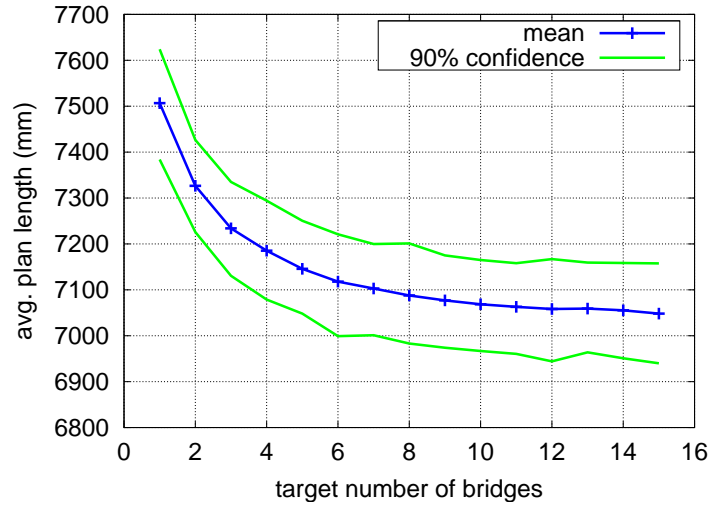
Fig. 14. The effect of multiple connection points in ERRT on plan length.
